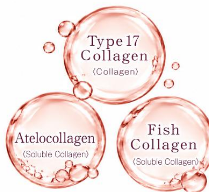
Triple Collagen
